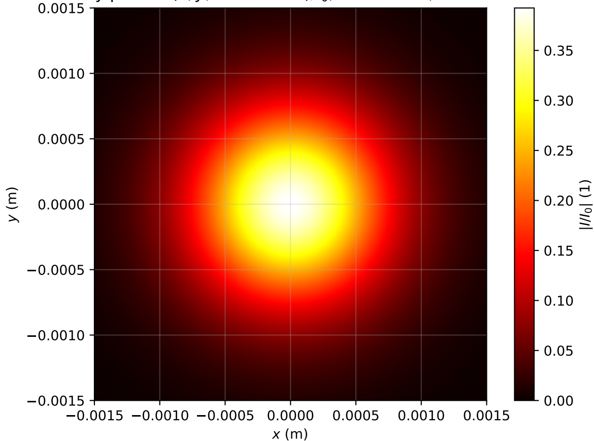
Intensity profile I(x, y, z = 3.981m)/I_0 , P_{in}=0.5P_{cr} , artificial time
